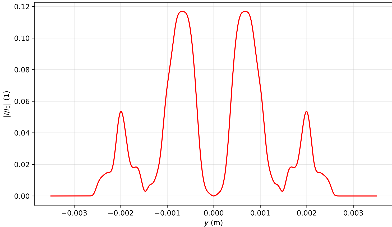
Intensity profile I(x=0, y, z=2.786)/I_0 , P_{in}=9.0P_{cr} , artificial time
